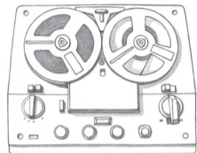
Band
