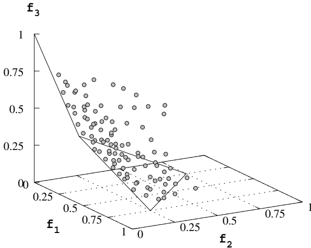
Figure 6.27. The SPEA2 population of non-dominated solutions on test problem DTLZ8.
