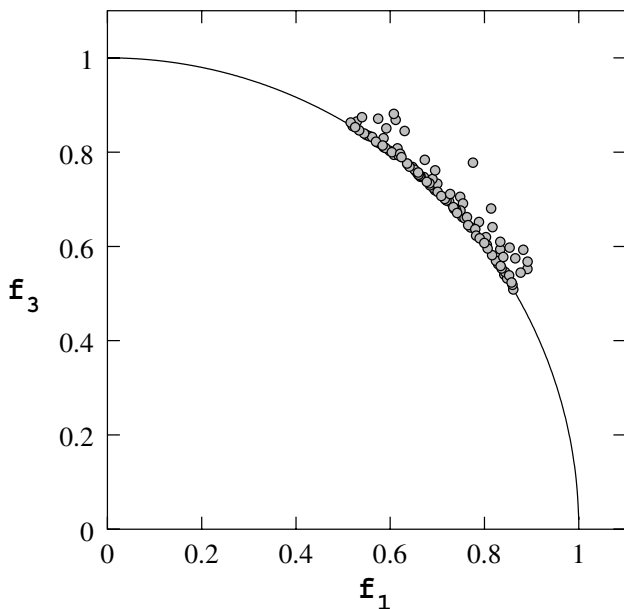
Figure 6.28. The NSGA-II population on test problem DTLZ9.
